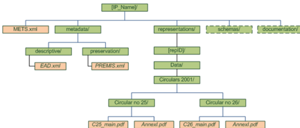
Figure 8 - Folder structure of the SMURF ERMS DIP
