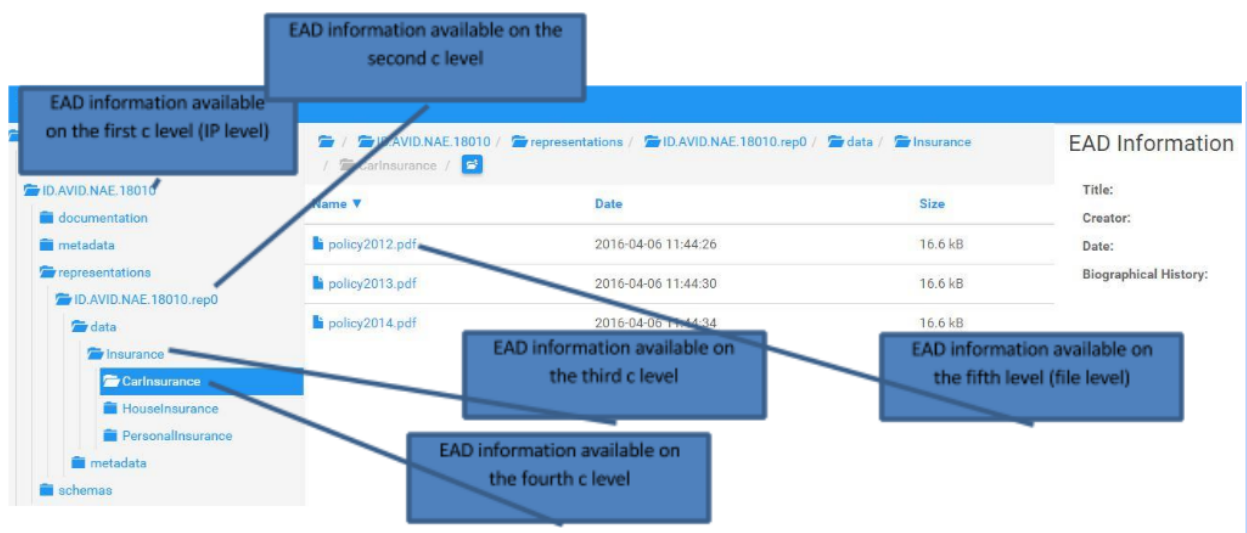
Figure 6 - Illustration of the E-ARK use of the EAD component tag <c>
